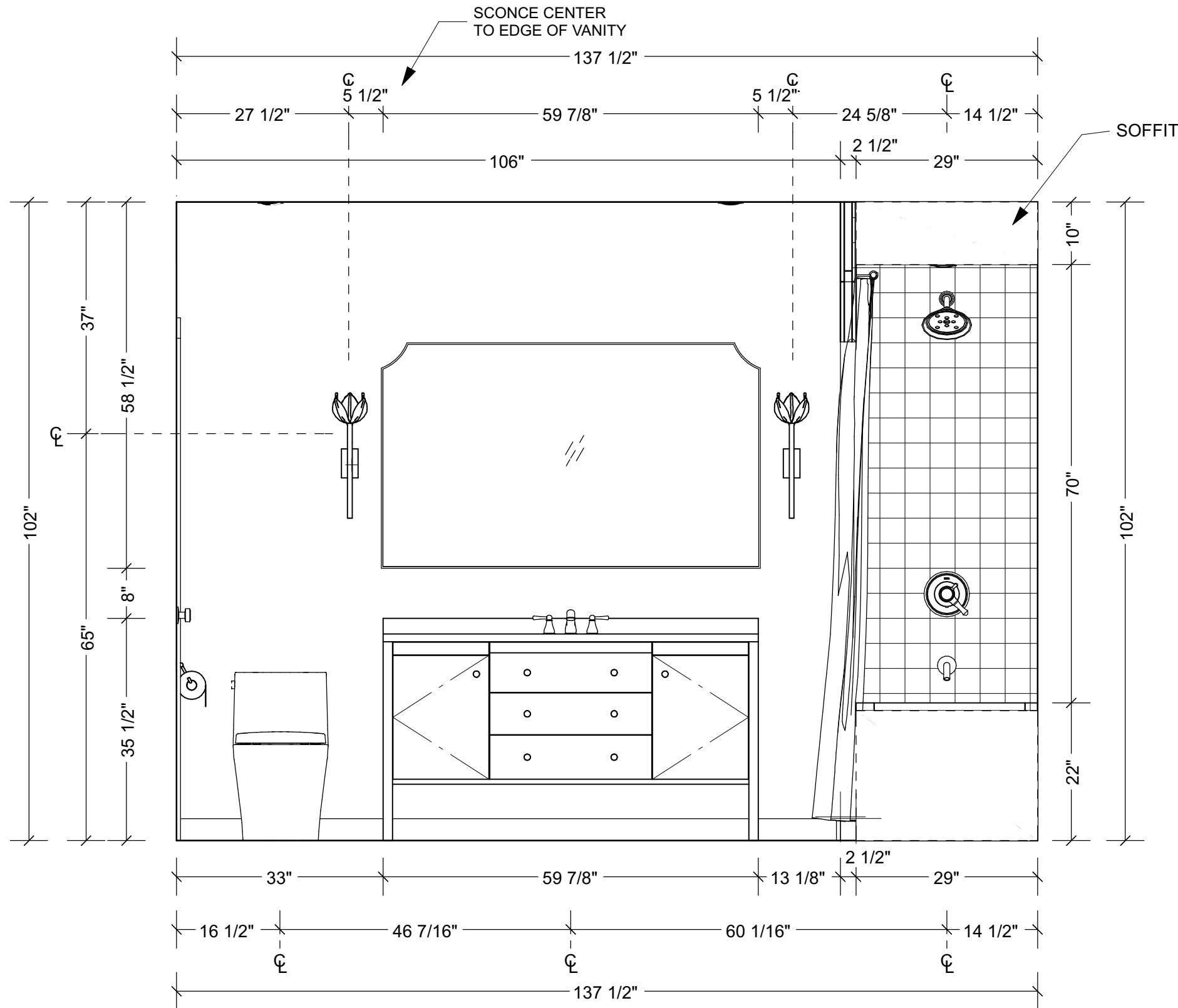
Bath 3 Elevation 1 5/8 in = 1 ft
