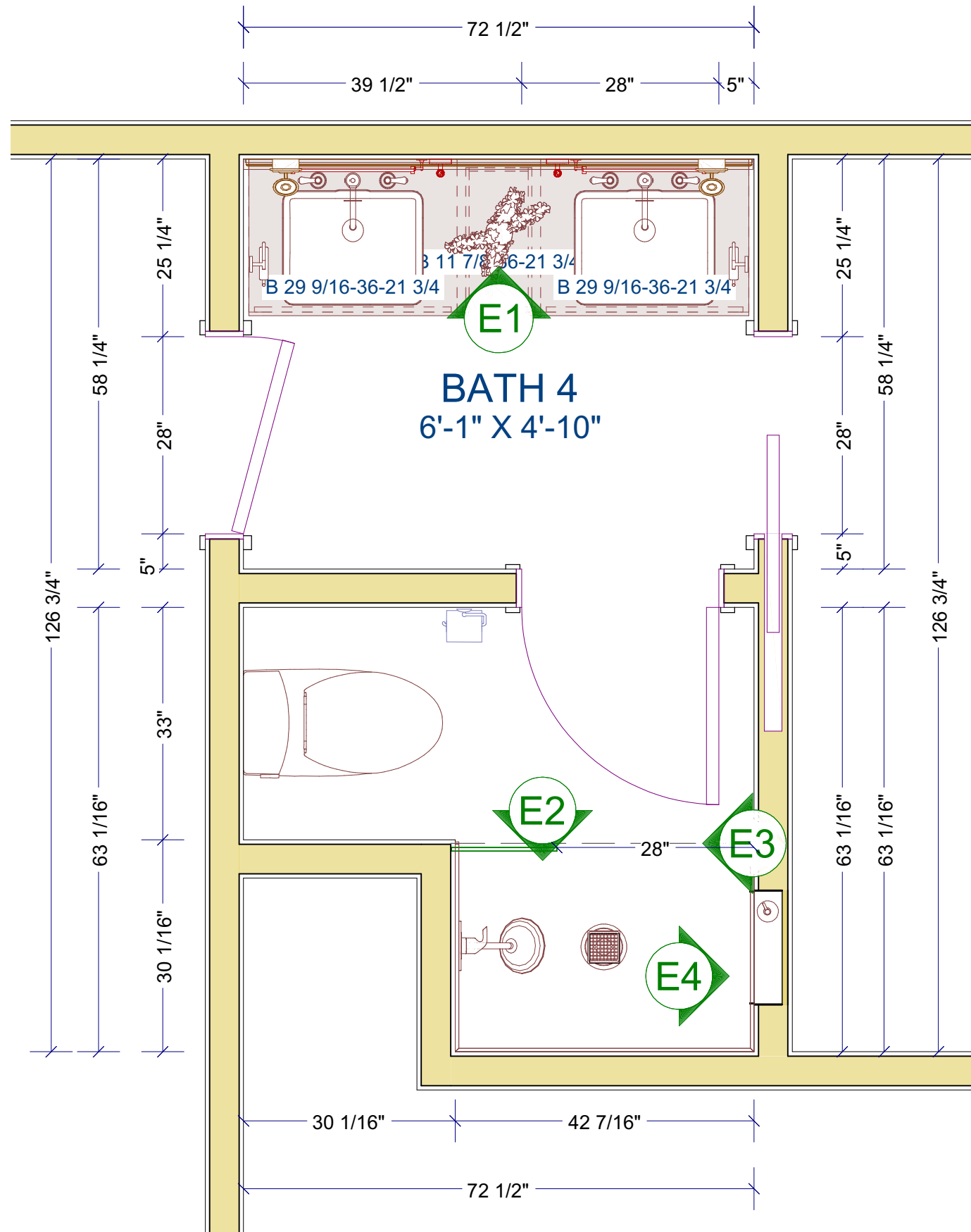
PLAN VIEW 5/8 in = 1 ft
